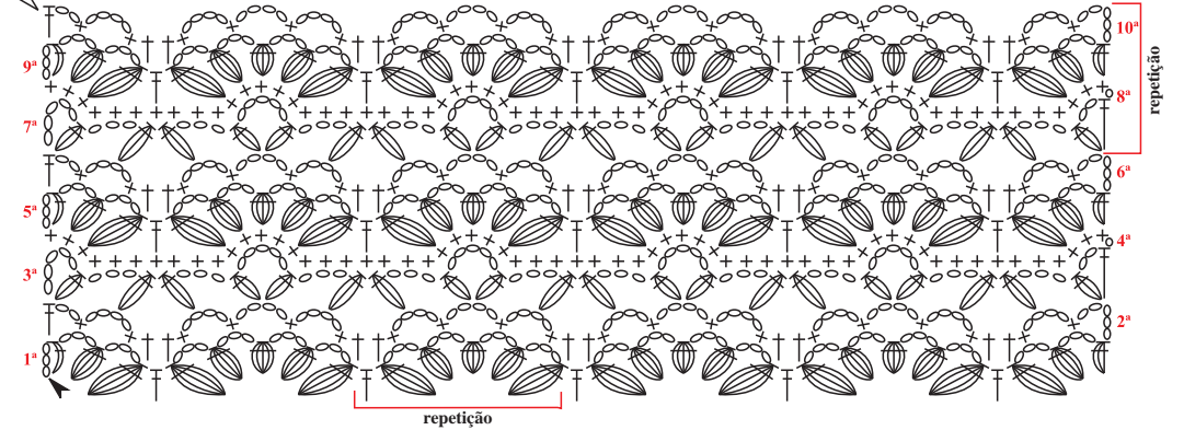
Diagrama 2 - Ponto fantasia (B)
